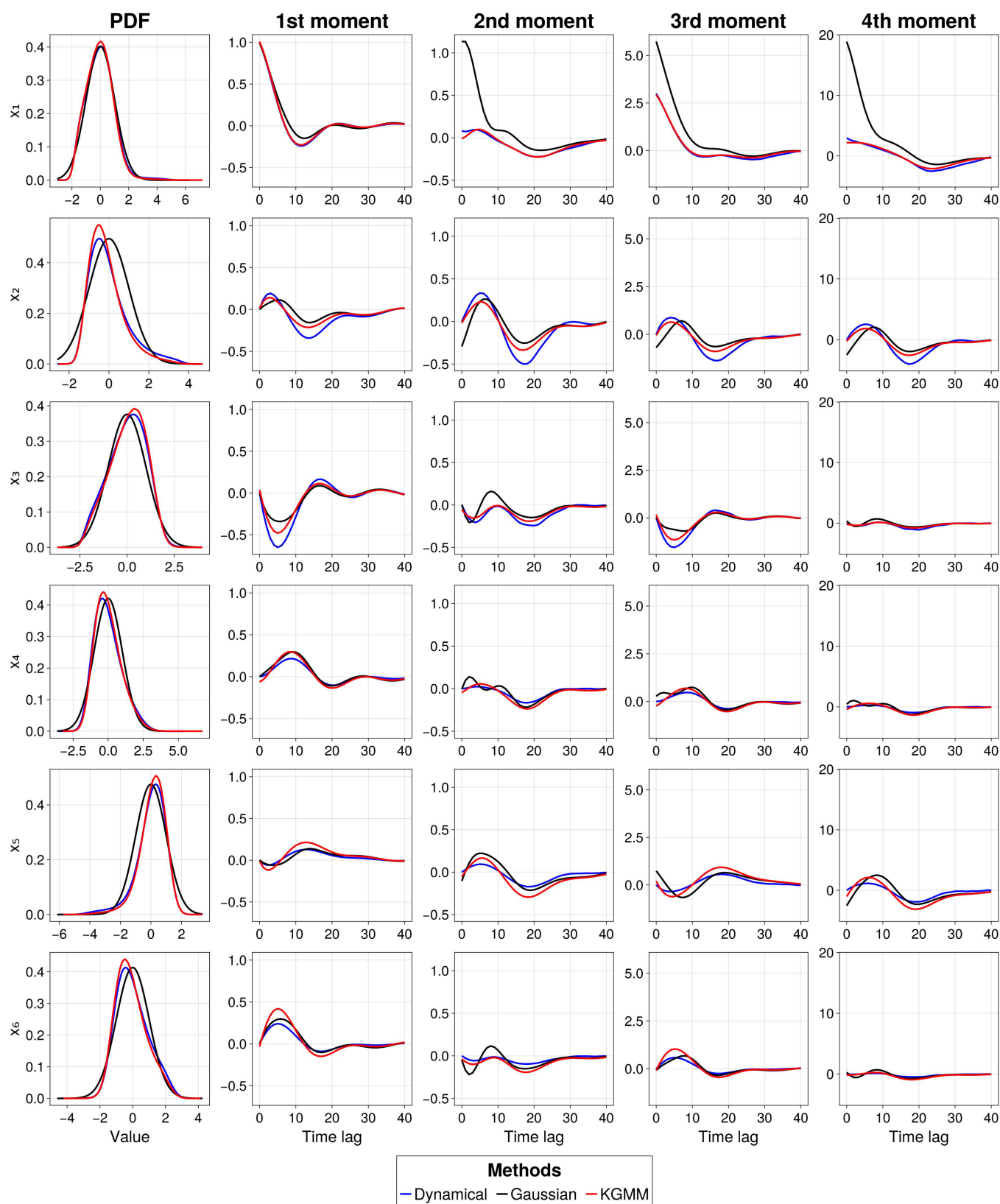
Fig. 3. Comparison of the unperturbed marginal steady-state PDFs (Left column) and response functions of the first four moments (remaining columns) for all six variables in the stochastic barotropic model. Results are shown for GFDT with score function estimated via KGMM (red), the linear Gaussian approximation (black), and numerical ensemble simulations (blue).
