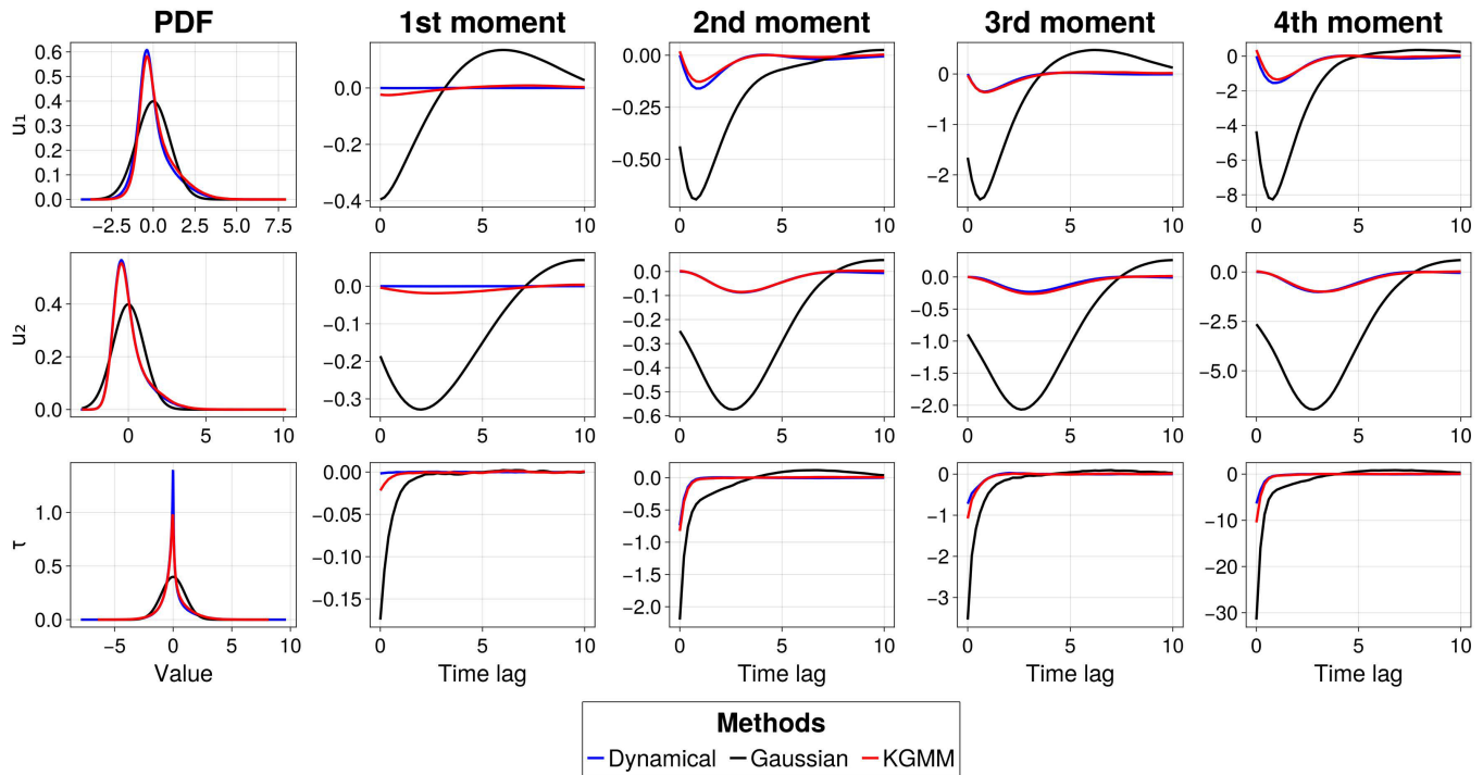
Fig. 2. Comparison of unperturbed marginal steady-state PDFs (leftmost column) and responses of the first four moments (remaining columns) in the slow-fast triad model for variables u_1 , u_2 , and \tau (rows). Response functions are shown as a function of time lag. Predictions obtained via GFDT using the KGMM-estimated score function (red), the Gaussian approximation (black), and numerical ground truth (blue) are reported.
