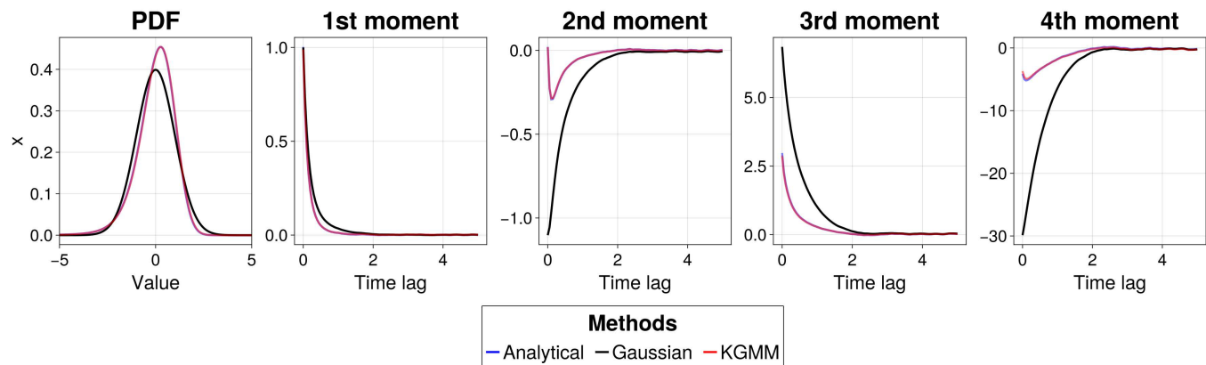
Fig. 1. Left: True unperturbed PDF (blue) compared with a normal Gaussian (black) and the PDF obtained integrating Eq. 15 with the KGMM score function (red). Right: Response functions predicted via GFDT. The true response functions (blue) are obtained using the analytic score function and are compared with the ones obtained using the KGMM score function (red) and the linear approximation (black). Note that the nonzero response of the second moment under the Gaussian approximation is due to the quasi-Gaussian framework used (Section 2.1), where the expectation is taken over the true non-Gaussian distribution.
