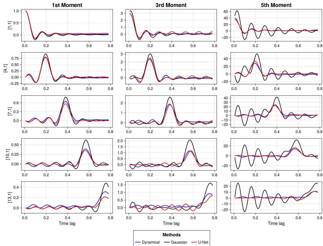
Fig. 4. Comparison of response functions for the 2D Navier-Stokes system with single-pixel perturbation. The plots show the response of the 1st, 3rd, and 5th moments across different time lags for five different observables, calculated using numerical integration (blue), U-Net score estimation (red), and linear Gaussian approximation (black). The U-Net method demonstrates superior agreement with the numerical ground truth compared to the linear approximation, particularly for higher-order moments where non-Gaussian effects are more significant.
